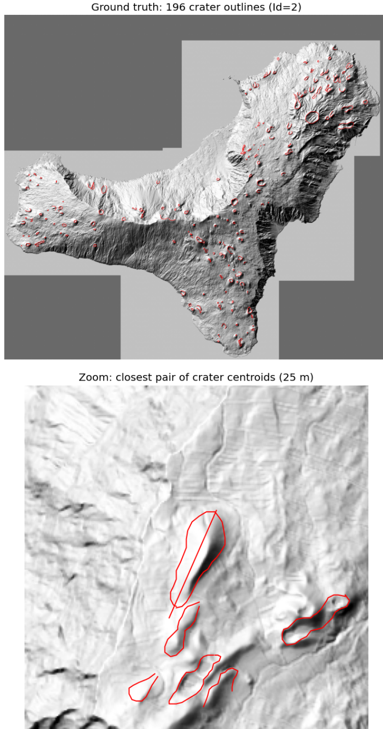
Figure 2: Ground truth on El Hierro. Top: the 196 crater outlines (Id= 2). Bottom: a zoom on the closest pair of crater centroids (25 m apart).
