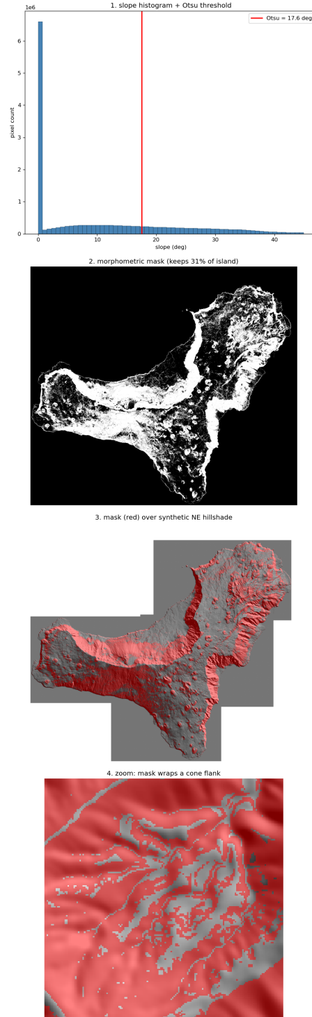
Figure 7: Data-driven morphometric mask on El Hierro. (1) Otsu threshold on the slope histogram ( 17.6^\circ ); (2) the resulting binary mask, keeping 31% of the island; (3) the mask (red) over the synthetic NE hillshade; (4) a zoom showing the mask wrapping a single cone flank.
