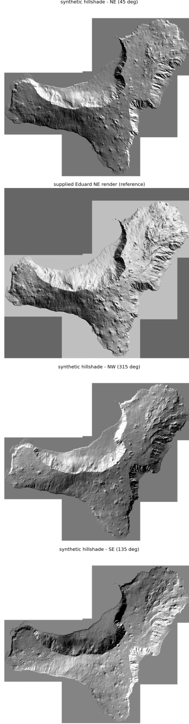
Figure 6: Synthetic hillshade on El Hierro from the steerable G_1 filters. Top: synthetic NE ( 45^\circ ) next to the supplied Eduard NE render (correlation 0.81). Bottom: the same basis re-steered to NW ( 315^\circ ) and SE ( 135^\circ ), showing the illumination rotating coherently.
