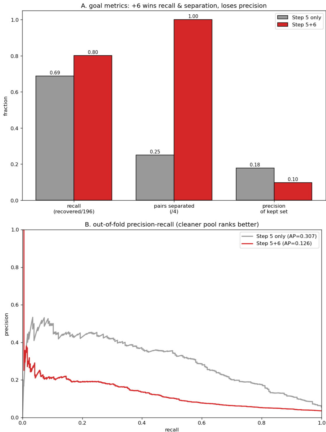
Figure 12: Step 7.5 on El Hierro. A : goal metrics — adding Step 6 (red) raises recall and takes pair separation from 1/4 to 4/4, while lowering the kept-set precision. B : the Step-5-only pool is cleaner and ranks better (higher AP), but cannot cover the merged cones; the union is the pool that delivers the separation.
