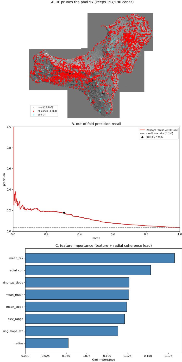
Figure 11: Step 7 on El Hierro. A : the Random Forest prunes the union pool \sim 5\times (grey: all 17,296 candidates; red: the ones kept; cyan: the 196 ground-truth craters). B : out-of-fold precision-recall curve (AP = 0.126) well above the candidate prior (0.035). C : feature importances — texture and radial aspect-coherence lead.
