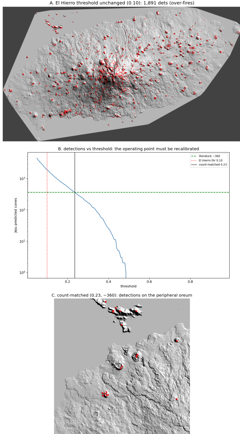
Figure 15: Step 9.5 on Jeju: zero-shot transfer of the El Hierro Random Forest. A : at the unchanged El Hierro threshold the model over-fires ( \sim 1,900 detections). B : detections vs threshold — the operating point must be recalibrated (literature \sim 360 in green, El Hierro threshold in red). C : at the count-matched threshold the detections fall on the peripheral oreum.
