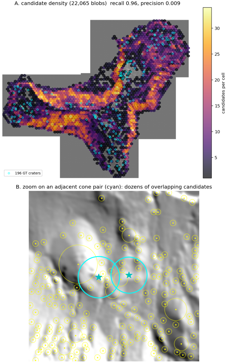
Figure 8: Step 4 on El Hierro. Top: density of the 22,065 permissive LoG candidates over the hillshade (recall 0.96, precision 0.009); the pool concentrates on steep terrain but is dominated by false positives. Bottom: zoom on an adjacent cone pair (cyan) surrounded by dozens of overlapping candidates, where no clean one-detection-per-cone assignment exists.
