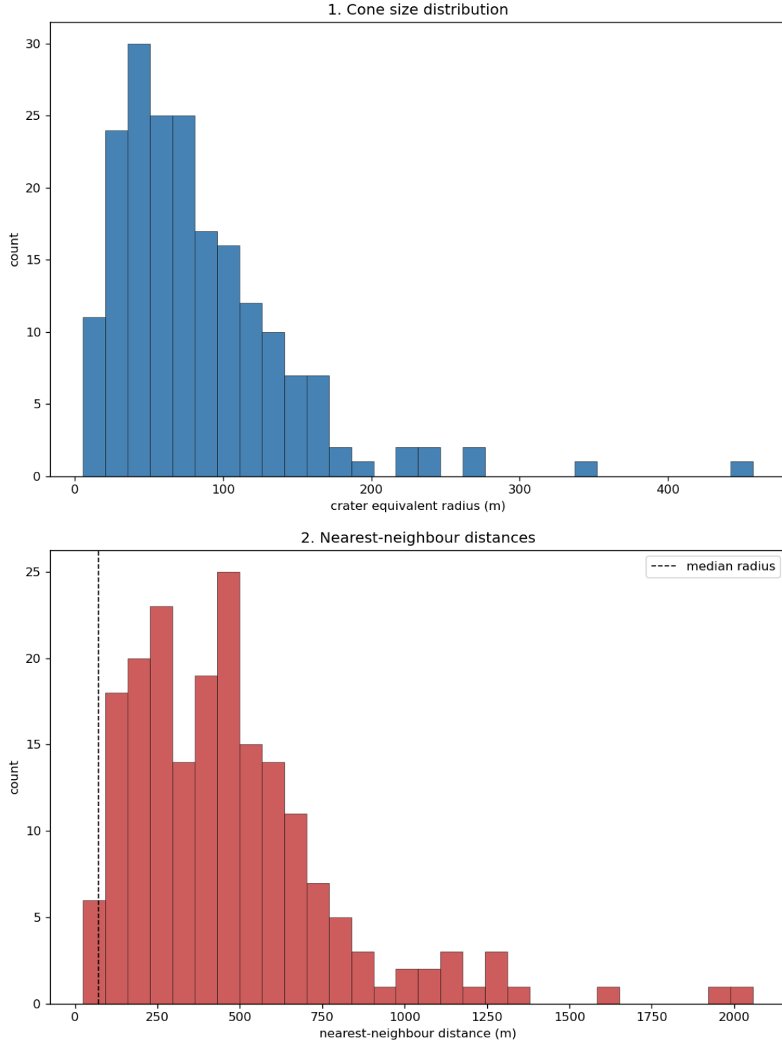
Figure 4: El Hierro crater statistics. Top: equivalent-radius distribution, used to set the LoG scale range. Bottom: nearest-neighbour distance distribution; the dashed line is the median radius, and the cones below it are the adjacent/nested cases.
