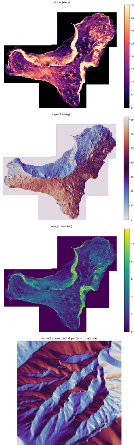
Figure 5: Morphometric channels derived from the El Hierro DEM: slope, aspect and roughness, plus a zoom of the aspect showing the radial pattern around a single cone.
