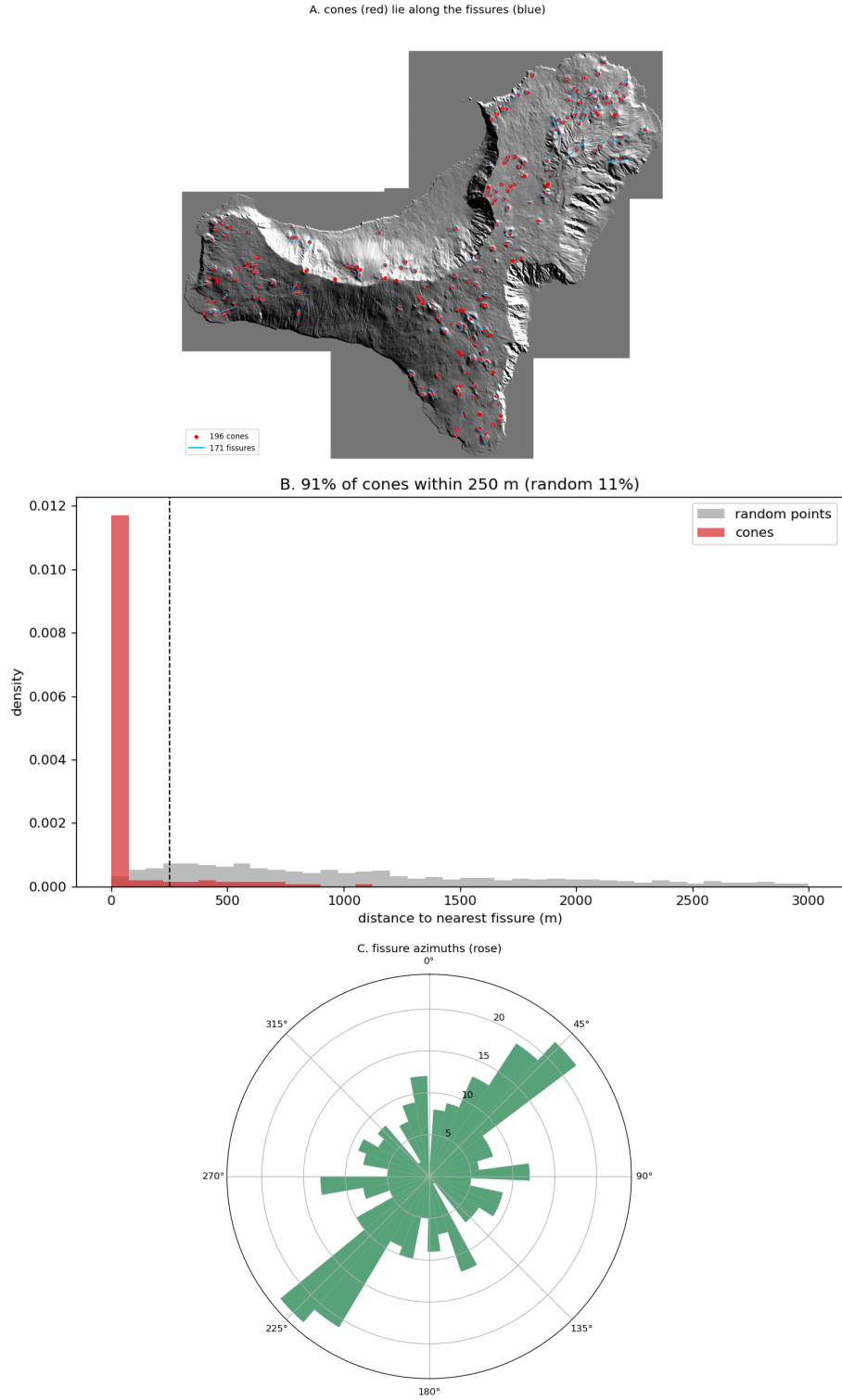
Figure 16: Step 10 on El Hierro. A : the mapped cones (red) lie along the eruptive fissures (blue). B : cone-to-nearest-fissure distance versus a random-points null — 91% of cones fall within 250 m of a fissure (random 11%). C : rose of fissure azimuths, showing the preferred swarm orientation.
