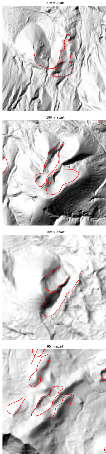
Figure 3: The adjacent/nested cases on El Hierro: the 4 crater pairs whose outlines overlap (8 craters). The watershed step is designed to split exactly these.
