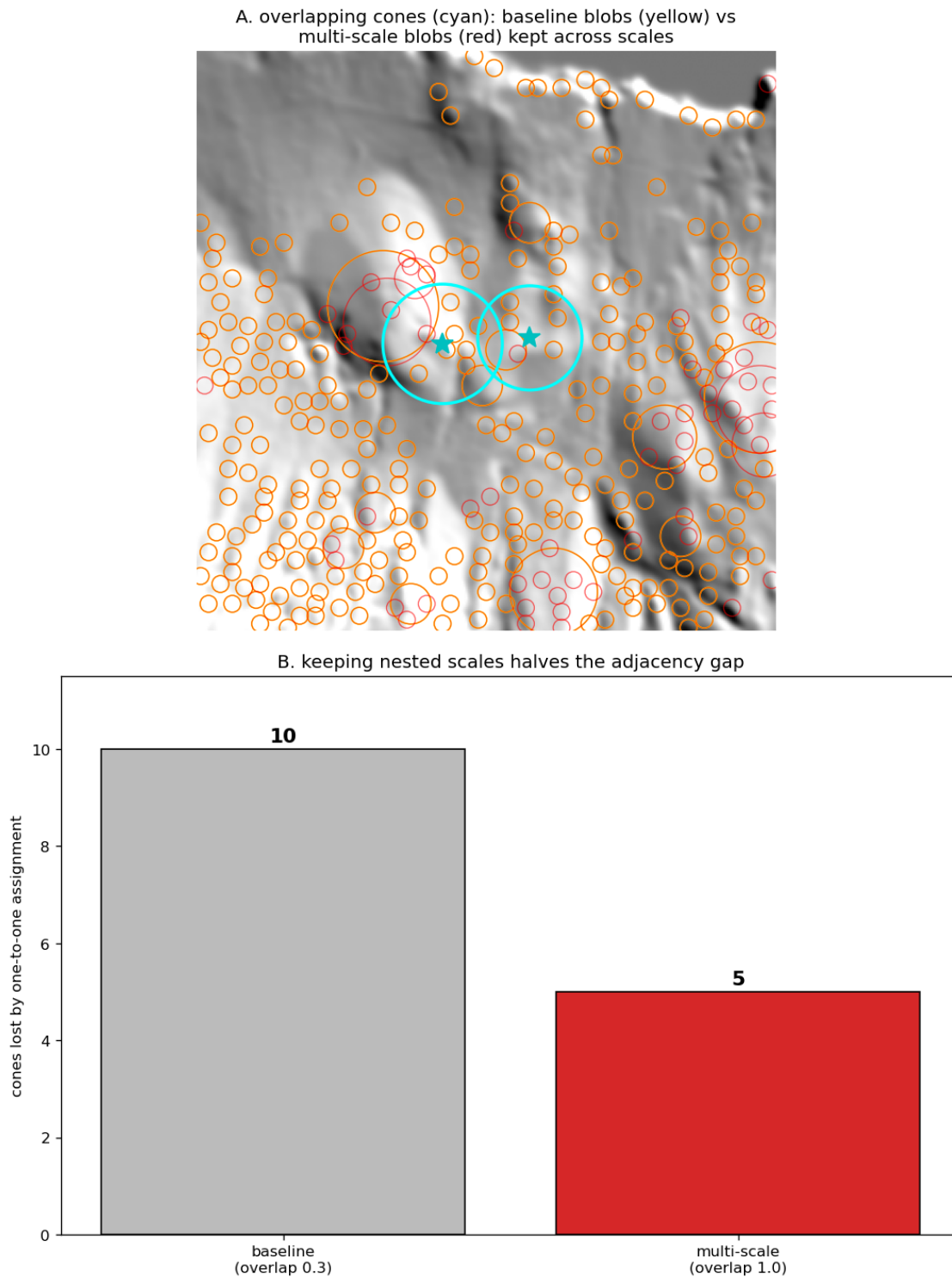
Figure 10: Step 6 on El Hierro. Top: zoom on an overlapping cone pair (cyan); the yellow circles are the Step 4 baseline blobs and the red circles the extra multi-scale responses kept by overlap = 1.0. Bottom: the strict one-detection-per-cone assignment loses 10 cones with the baseline pool but only 5 once nested scales are retained.
