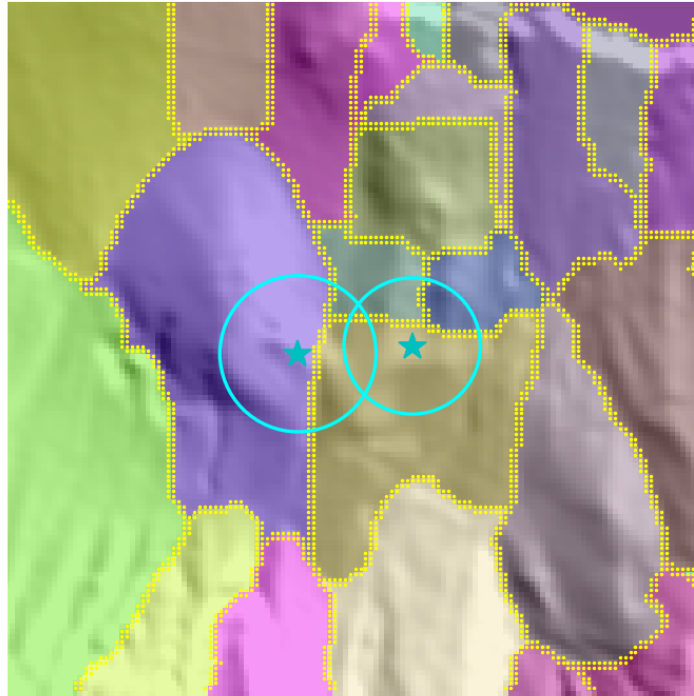
B. an adjacent pair LoG merged: watershed yields 2 basins (boundary in yellow)
