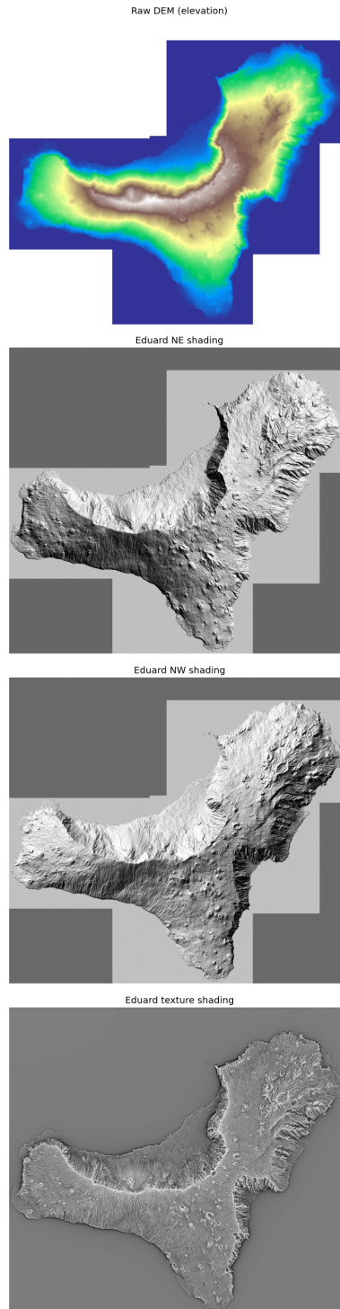
Figure 1: El Hierro: the raw DEM (top) is visually flat, while the Eduard renderings reveal the conical landforms.
